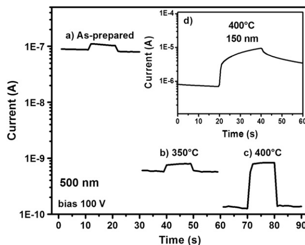
Fig. 6. Photoresponse of the \beta - \text{In}_2\text{S}_3 thin films with 39 h of deposition, a) as-prepared, b) annealed at 350 °C in \text{N}_2 , and c) annealed at 400 °C in \text{N}_2 . Inset d): photoresponse of the \beta - \text{In}_2\text{S}_3 thin film with 16 h of deposition after annealing at 400 °C.
