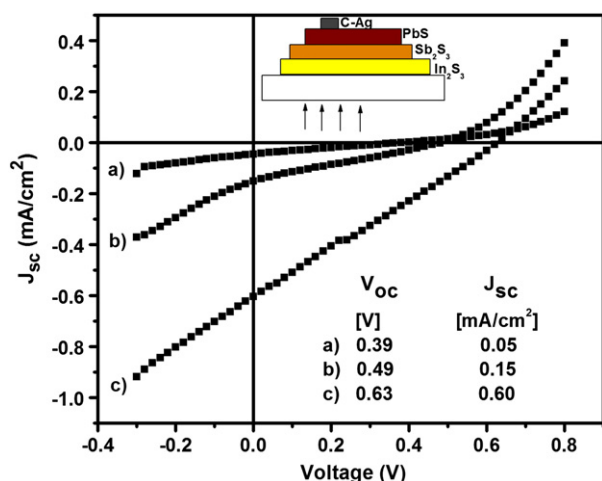
Fig. 7. J–V characteristics of the \text{SnO}_2\text{:F}/\text{In}_2\text{S}_3/\text{Sb}_2\text{S}_3/\text{PbS}/\text{C-Ag} photovoltaic structures using a) an as-prepared \text{In}_2\text{S}_3 layer with a thickness of 200 nm; b) an as-prepared \text{In}_2\text{S}_3 layer with a thickness of 165 nm; and c) an \text{In}_2\text{S}_3 layer with a thickness of 157 nm after thermal treatment at 350 °C in \text{N}_2 .
